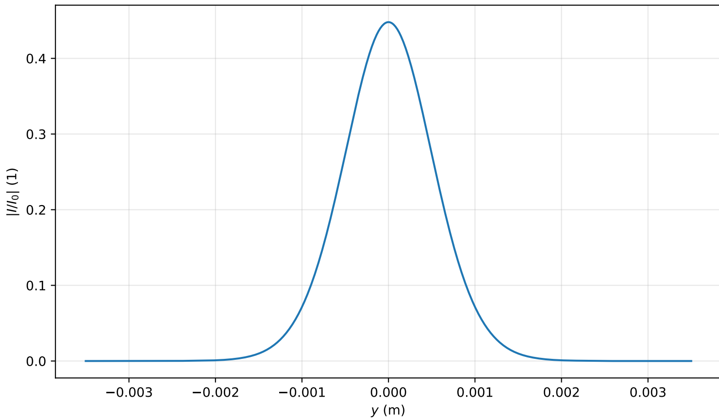
Intensity profile I(x=0, y, z=2.866)/I_0 , P_{in}=0.3P_{cr} , artificial time
